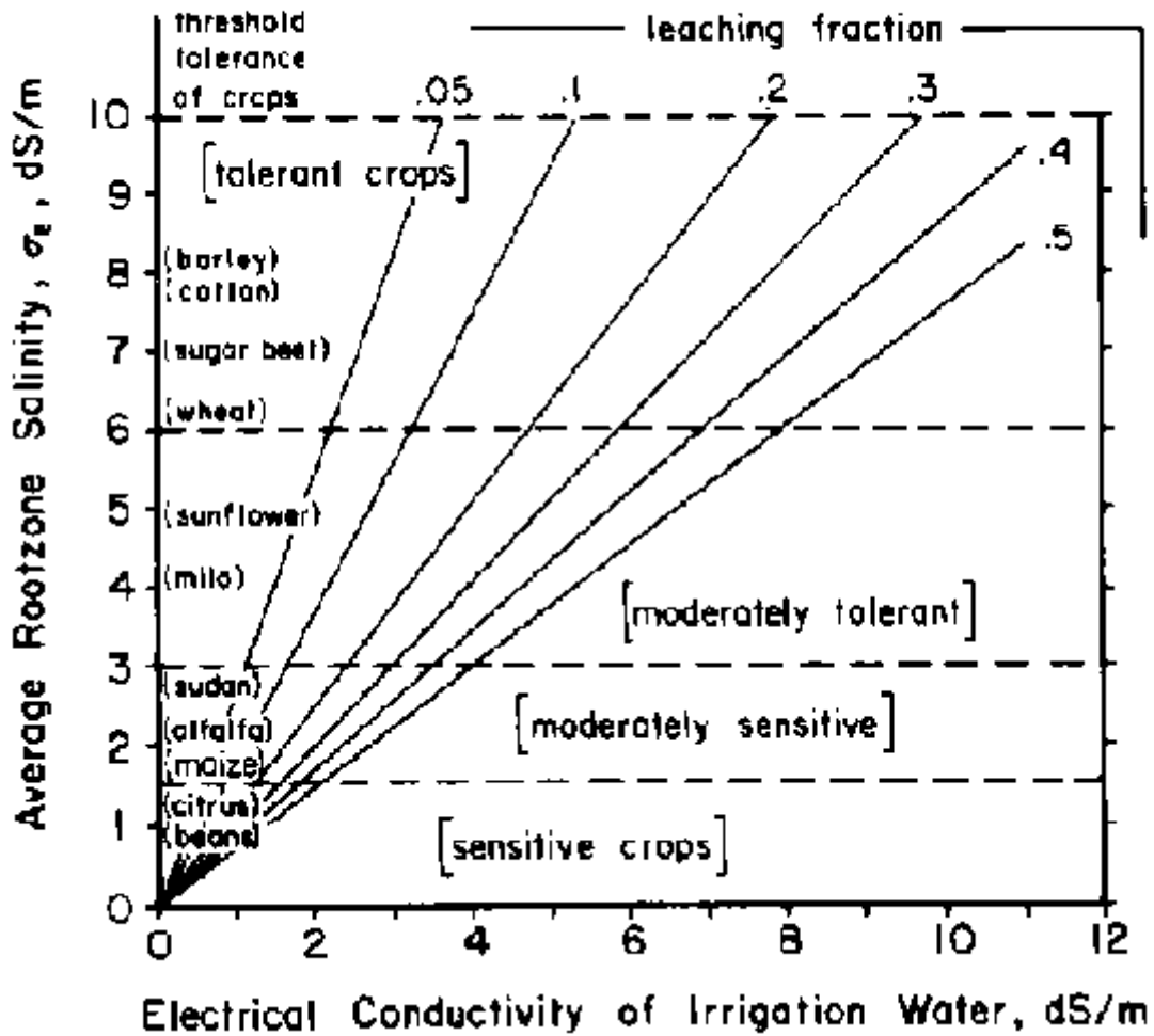
FIGURE 9 Relationships between water-uptake-weighted salinity (saturation extract basis), EC of irrigation water and LF for conditions of high-frequency irrigation
